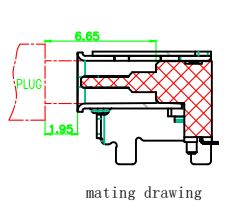
mating drawing
