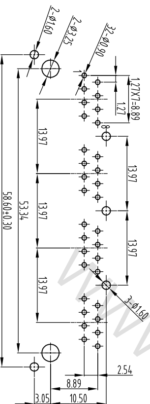
PCB LAYOUT/TOP VIEW
