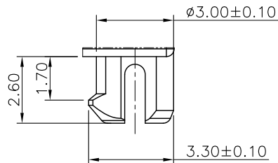
DETAIL "X" SCALE 4:1
