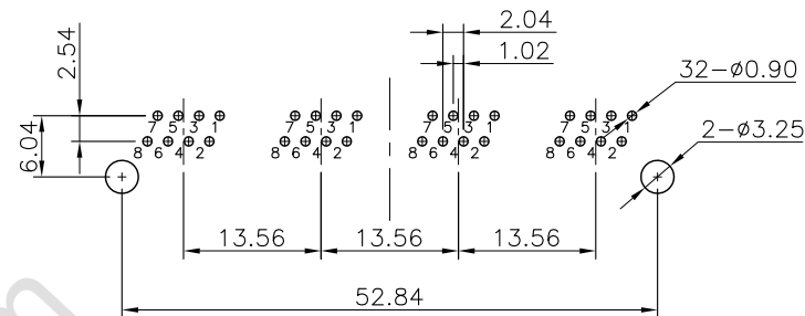
RECOMMENDED PCB LAYOUT TOP VIEW (TOL:±0.05)
