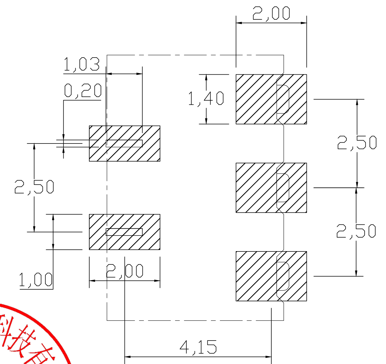
RECOMMENDED PCB LAYOUT TOP VIEW(. XX ± 0.05)
