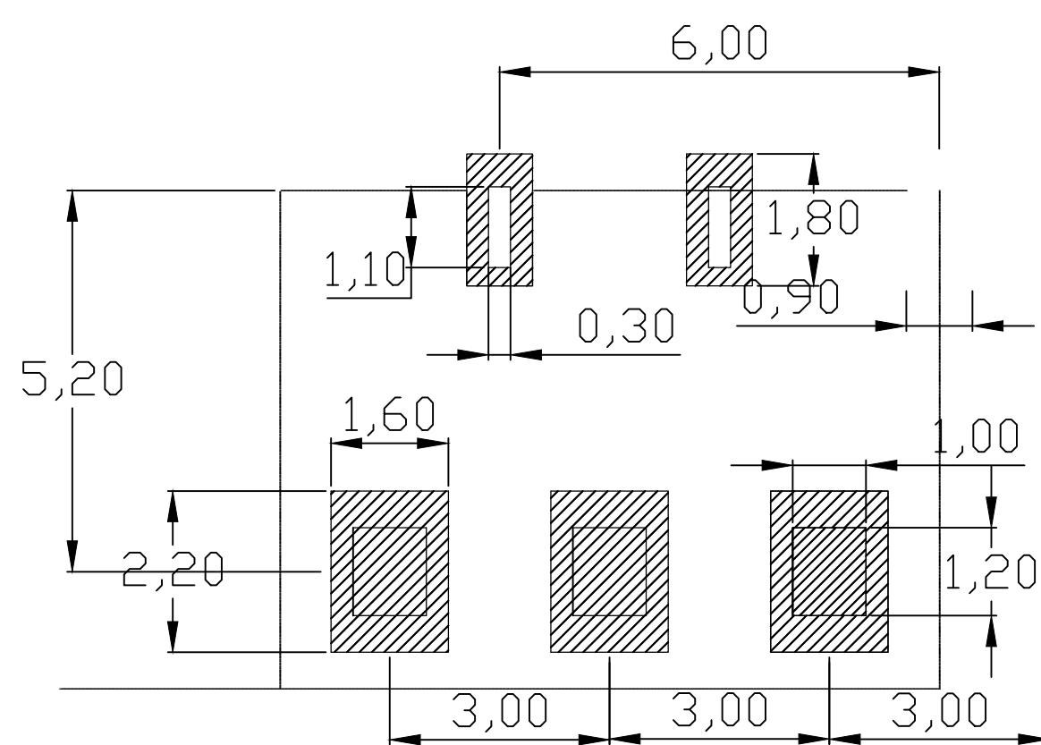
RECOMMENDED PCB LAYOUT TOP VIEW(. XX±0.05)
