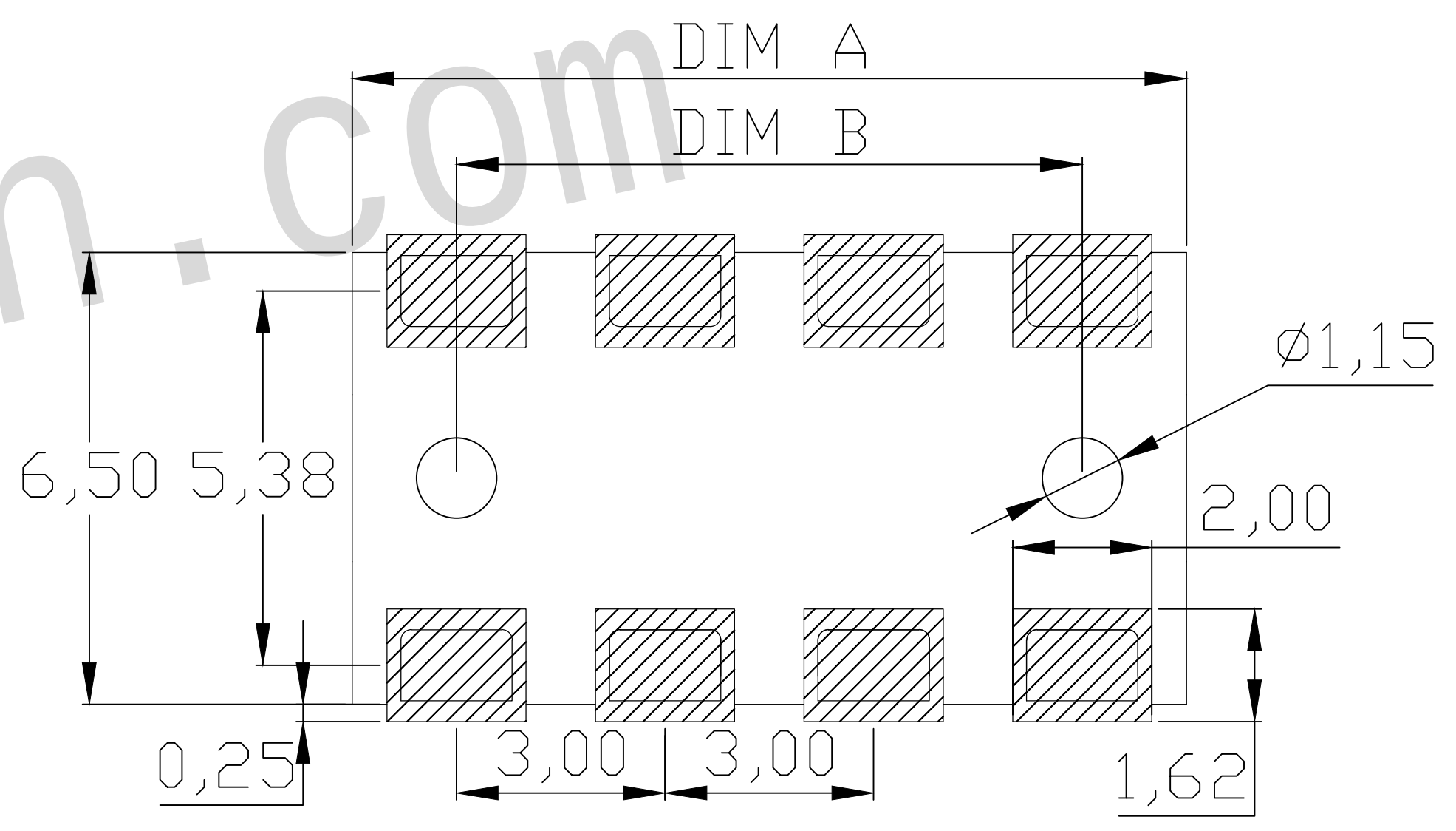
RECOMMENDED PCB LAYOUT TOP VIEW(.XX±0.05)
