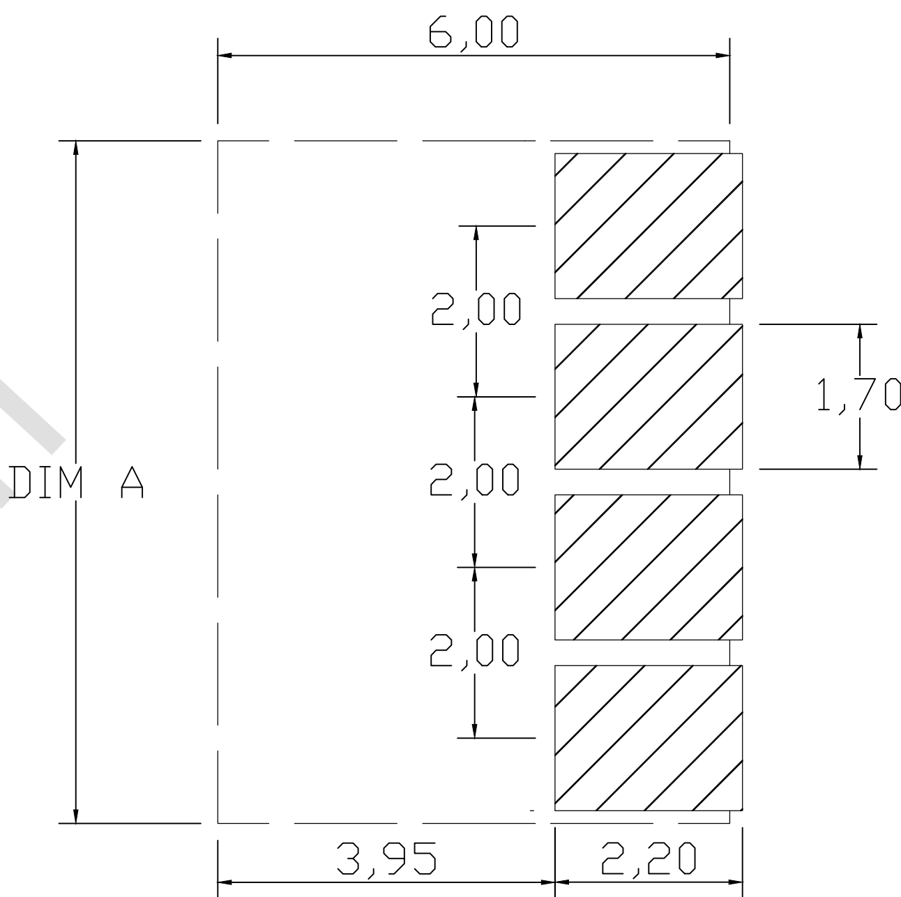
RECOMMENDED PCB LAYOUT TOP VIEW(. XX±0.05)
