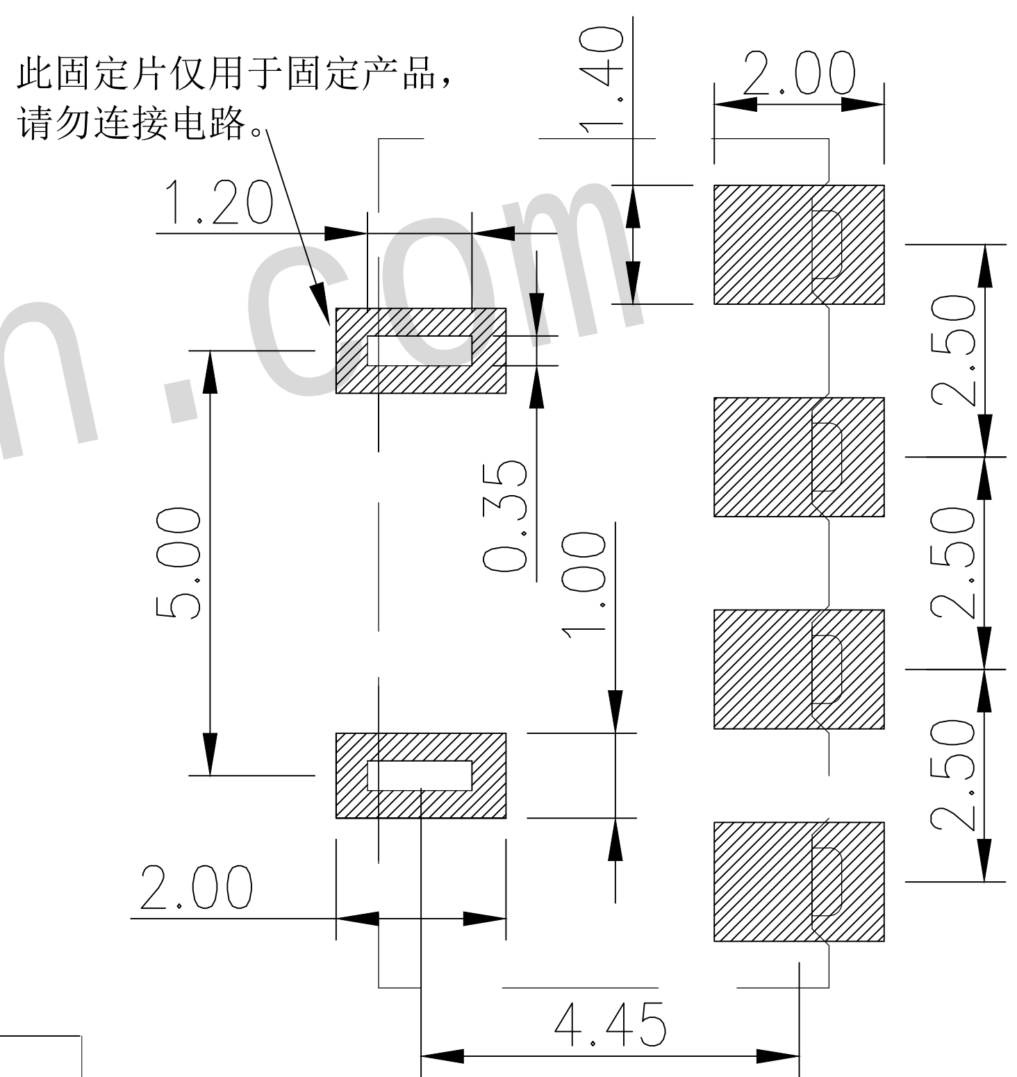
RECOMMENDED PCB LAYOUT TOP VIEW (.XX±0.05)
