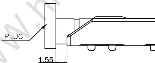
PLUG MATE DRAWING
