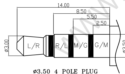
4 POLE PLUG
