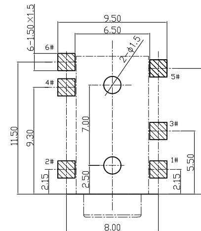
RECOMMEND PCB LAYOUT TOLERANCE ±0.05
