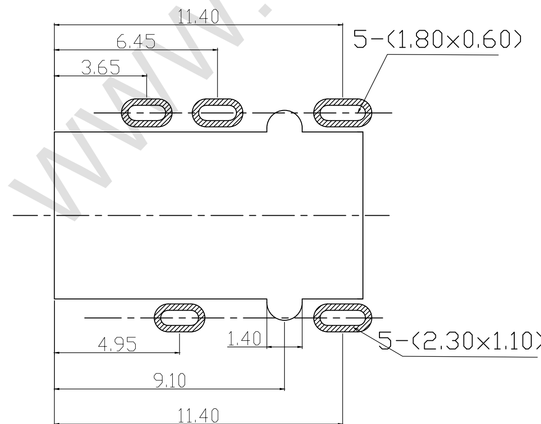
RECOMMEND PCB LAYOUT TOLERANCE \pm 0.05
