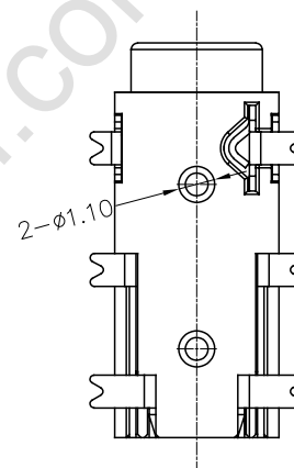
P.C.B LAYOUT TOP VIEW
