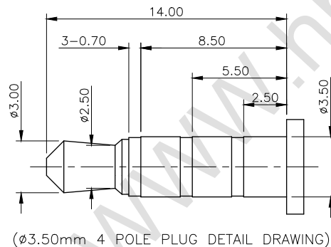
(ø3.50mm 4 POLE PLUG DETAIL DRAWING)
