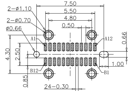
RECOMMEND P.C.B LAYOUT (COMPONENT SIDE) TOLERANCE FOR PCB LAYOUT IS \pm 0.05
