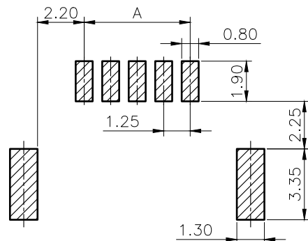
Recommended P.C.Board Layout General Tolerance: \pm 0.1
