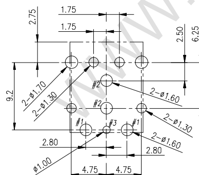
RECOMMENDED P.C.B LAYOUT TOP VIEW (TOLERANCE: \pm 0.05 )
