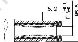
MATING PLUG
