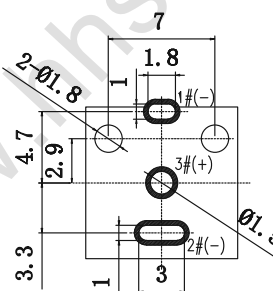
PCB LAYOUT TOP VIEW (TOLERANCE: \pm 0.05 )
