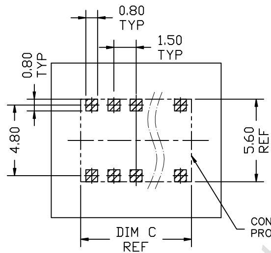
RECOMMENDED PCB LAYOUT TOLERANCE: \pm 0.10
