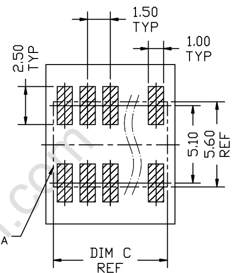
RECOMMENDED FPC LAYOUT TOLERANCE: \pm 0.10
