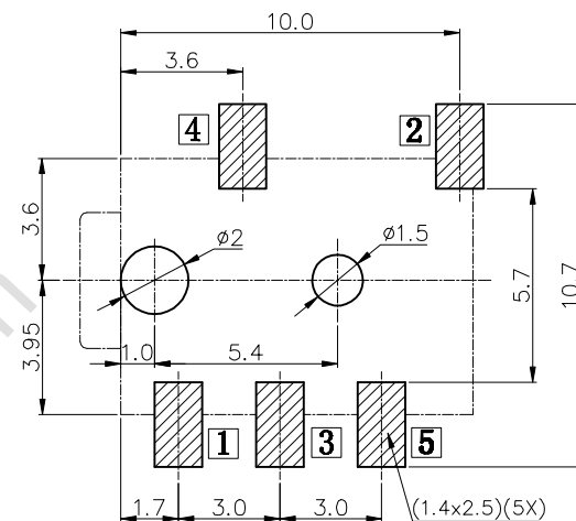
PCB HOLES(TOP VIEW) t=1.0mm NOTE: GENERAL TOLERANCE: ±0.05mm
