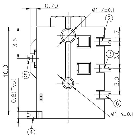
RECOMMENDED PLUG Ø2.5 3-POLE STANDARD PLUG
