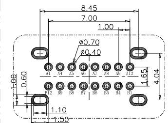
RECOMMEND P.C.B LAYOUT TOLERANCE UNSPECIFIED ±0.05mm
