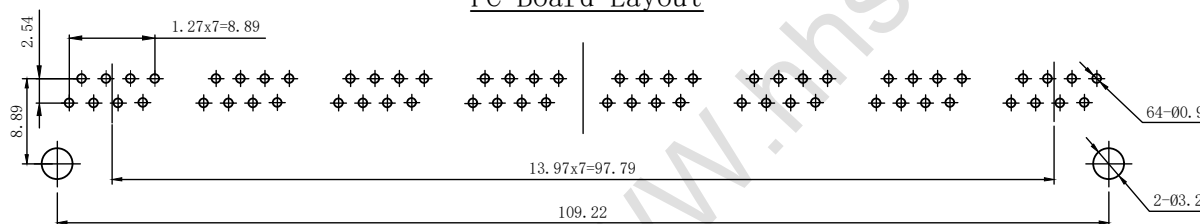
PC Board Layout
