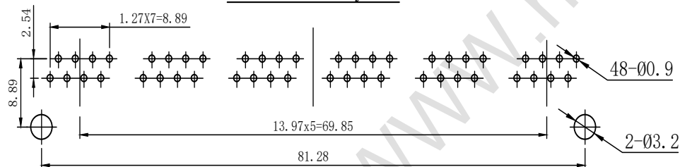
PC Board Layout
